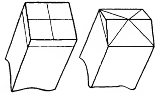
FIG. 388. POST LAID OUT FOR TOP TAPER.
